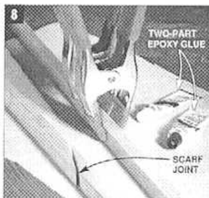
JOIN STRIPS of ash for the inwales and outwales with a "scarf joint," a low-angled lap joint. Glue the joint with epoxy.
