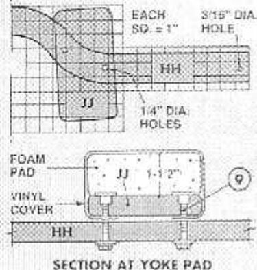
FIG. C YOKE DETAIL
