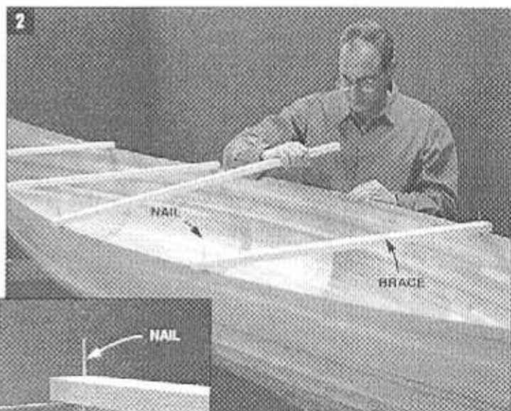
WOOD BRACES with nails at the ends keep the hull from bowing in when you're not working on it. Use the molds to determine the nail spacing.
