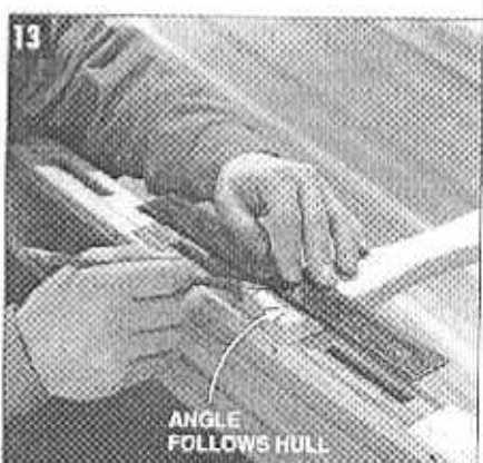
MARK THE THWARTS so they fit the angle of the hull, cut them, then bolt them underneath the inwales with stainless steel bolts.
