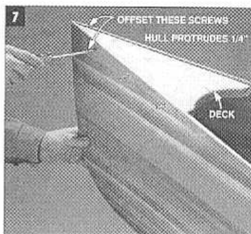
ATTACH THE ASH DECKS to the hull with stainless steel screws. Offset the two screws nearest the ends so they don't interfere with each other.
