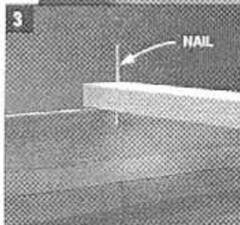
WOOD BRACES with nails at the ends keep the hull from bowing in when you're not working on it. Use the molds to determine the nail spacing.
