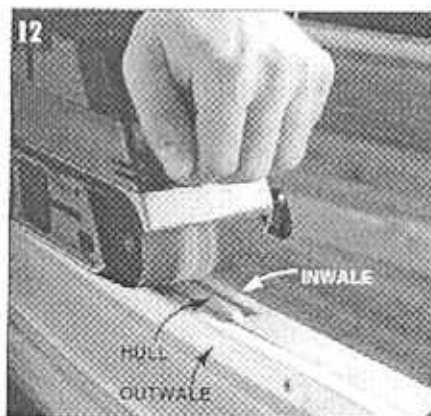
SAND THE GUNWALES FLUSH with a belt sander, removing the 1/4 in. of hull that protrudes. Hold the sander as flat as possible while you sand.
