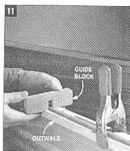
CLAMP ON THE OUTWALE and get it aligned, then screw it on. A notched block of wood helps get the outwale and inwale lined up evenly.
